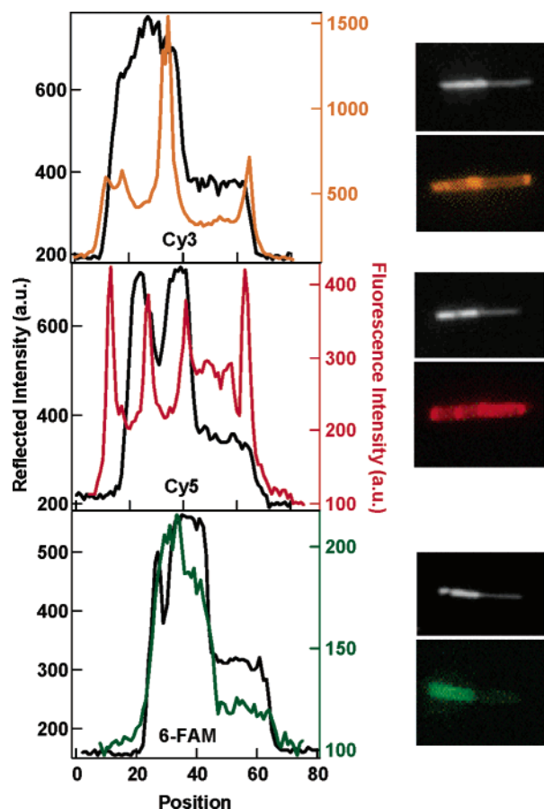
Figure 7. Line scans with corresponding reflectance (top) and fluorescence (bottom) images of nanowires coated with 5' thiol, 3' fluorophore, 34-base molecular beacon probes, for three fluorophores. The black traces (reflectance) correspond to the left axis, and the colored traces (fluorescence) correspond to the right axis.
