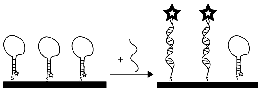
Scheme 3. Hybridization of Surface-Bound Molecular Beacon Probes
