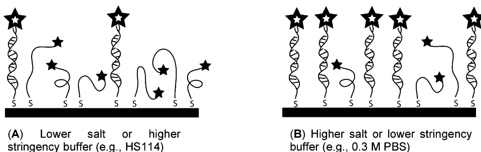
Scheme 2. Hybridization Efficiency Impacts Average Dye–Metal Separation
