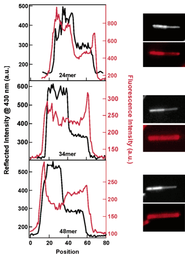
Figure 6. Line scans and corresponding reflectance (top) and fluorescence (bottom) images of half Ag/half Au nanowires coated with 5' thiol, 3' TAMRA probe oligonucleotides of different lengths. The 24-base probe did not have secondary structure; however the 34- and 48-base probes were molecular beacons with self-complementarity at the 5' and 3' ends. Unlabeled complementary DNA was present in all cases to extend the probes from the surface. The black trace (reflectance) corresponds to the axis on the left, and the red trace (fluorescence), to the axis on the right.
